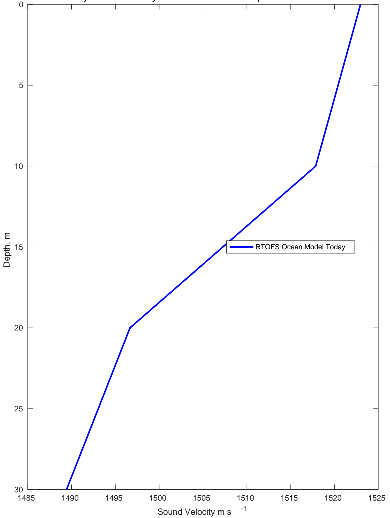
Sound Velocity Profile for Vineyard Wind GB48 on 07-Sep-2022 00:00:00
